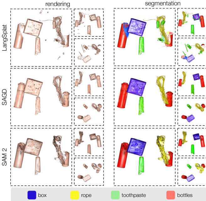
Fig. 1: Comparison of LangSplat, SAGD, and SAM 2 on the backpack dataset. Each row shows the renderings of the reconstructed scene (left) alongside the corresponding semantic segmentation (right).
